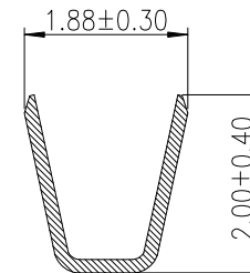
SECTION Y-Y
