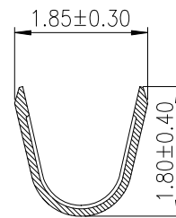
SECTION X-X
